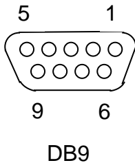
DB9 Female viewed from the pin side. Wiring is on opposite side.
